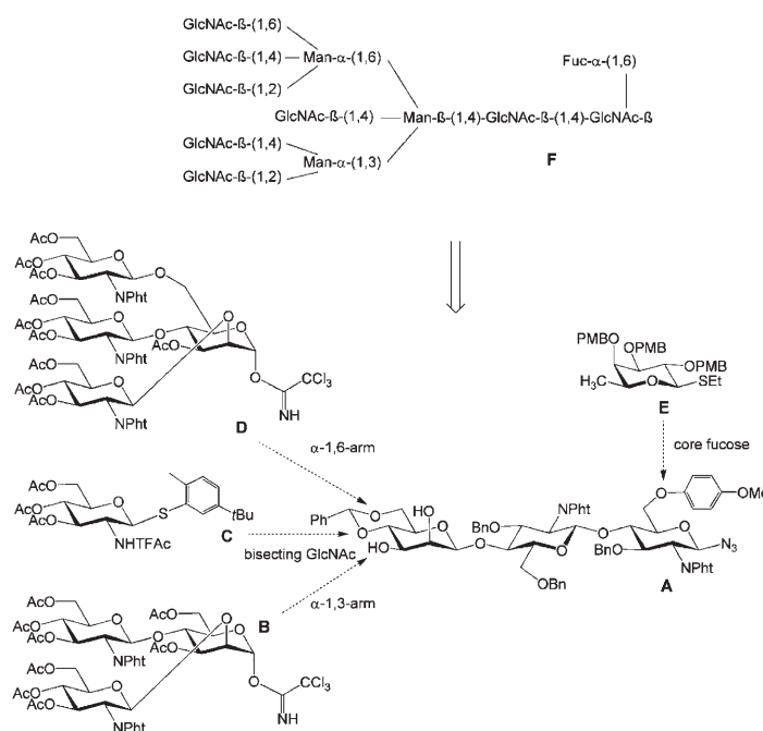
Scheme 1. Retrosynthesis of pentaantennary N-glycans with bisecting GlcNAc and core fucose groups. Ac = acetyl, Bn = benzyl, Pht = phthalimido, PMB = p -methoxybenzyl, TFAc = trifluoroacetyl.
