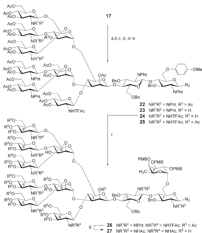
Scheme 5. a) D , \text{BF}_3 \cdot \text{OEt}_2 , \text{CH}_2\text{Cl}_2 , -10^\circ\text{C} , MS (4 Å), ( 22 , 9%); b) 8 , NIS, \text{TfOH} , \text{CH}_2\text{Cl}_2 , -30^\circ\text{C} , MS (4 Å) ( 22 , 8%); c) 9 , NIS, \text{TfOH} , \text{CH}_2\text{Cl}_2 , -30^\circ\text{C} , MS (4 Å) ( 23 , 31%); d) 10 , NIS, \text{TfOH} , \text{CH}_2\text{Cl}_2 , -30^\circ\text{C} , MS (4 Å) ( 24 , 47%); e) 11 , NIS, \text{TfOH} , \text{CH}_2\text{Cl}_2 , -30^\circ\text{C} , MS (4 Å) ( 25 , 38%); f) 1. CAN, \text{CH}_3\text{CN} , toluene, \text{H}_2\text{O} , 82%; 2. E, \text{CuBr}_2 , \text{Bu}_4\text{NBr} , \text{CH}_2\text{Cl}_2 , DMF, 75%; g) 1. ethylenediamine, n\text{BuOH} , 80^\circ\text{C} ; 2. \text{Ac}_2\text{O} , pyridine; 3. \text{MeNH}_2 (40% in \text{H}_2\text{O} ) (1–3., 59%).
